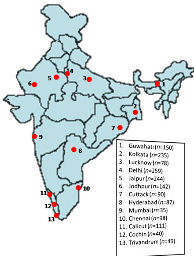
Fig. 1 Map of India showing location of centers in the country, which recruited patients in the study. Data within the parenthesis denote number of patients recruited by each place
